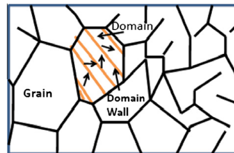
Fig. 12. Schematic diagram of defect dipoles and domain wall motion in the PZT–PDMS composite.
