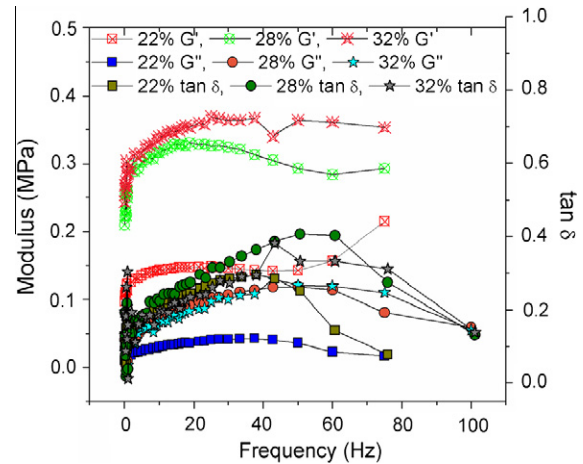
Fig. 7. Storage ( G' ) and loss ( G'' ) modulus and material loss factor ( \tan \delta ) of the hard PZT–PDMS composites as a function of frequency.
