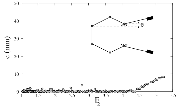
Fig. 16. Variation of link length e with the second objective function. The value of e is almost constant for the different optimal configurations with a low value of force transformation ratio and can be fixed at its lower bound. However, for very high-force transformation ratios (above 4.5), the value varies, more or less linearly, from 0 to 10.
