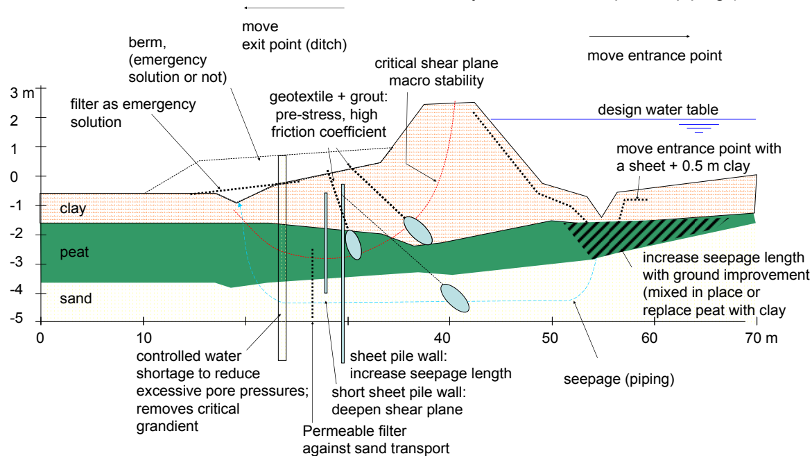
Figure 2. Case 1: levee improvement close to Genemuiden; In this drawing all possible solutions which were generated in a brainstorm for stability, piping and landscape problems are shown together.
