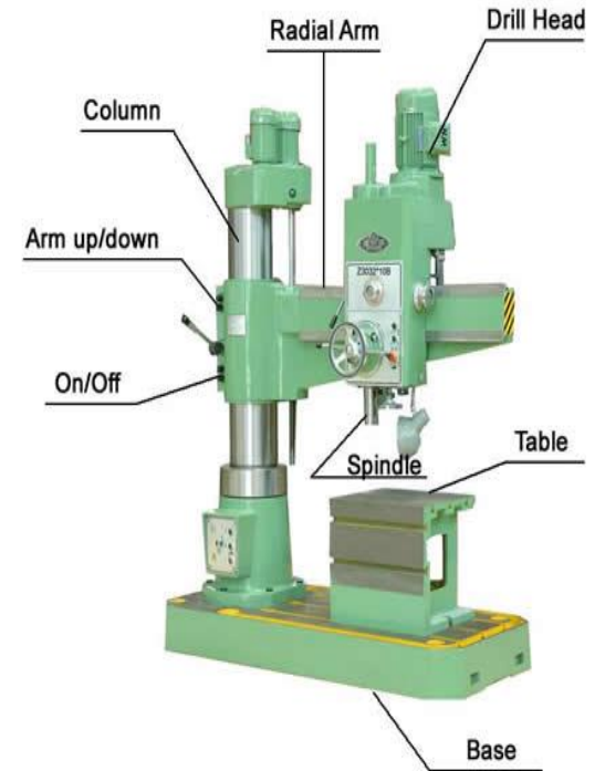
Drilling Machine
