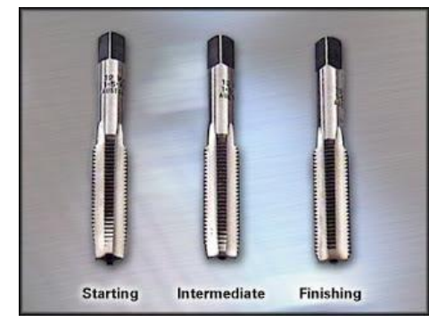
Taps
