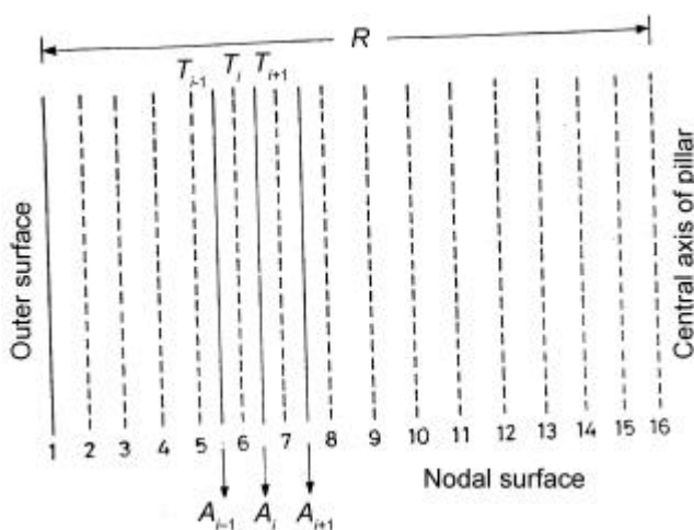
Figure 5. Schematic representation of the division of the pillar into segments for calculation purposes.
