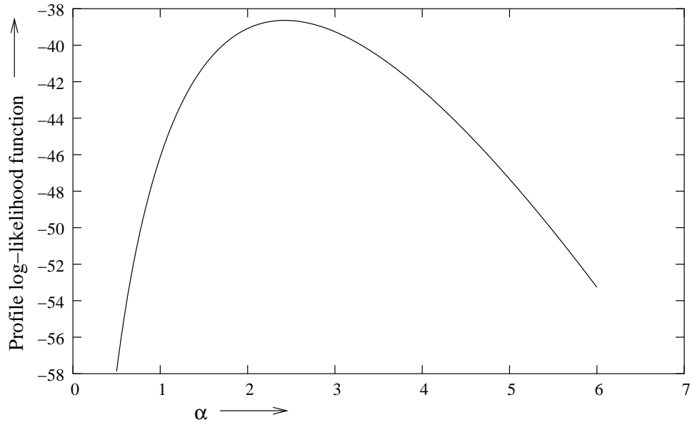
Figure 1: Profile log-likelihood function of \alpha for Type-I censored sample.
