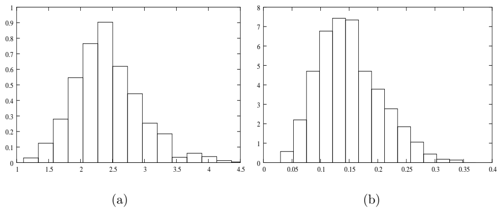
Figure 2: Histogram plots: (a) MCMC samples of \alpha (b) MCMC samples of \lambda
