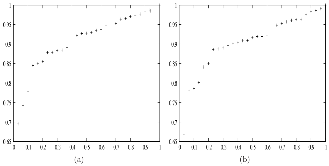
Figure 2: Scaled TTT plots of the marginals. (a) Shock, (b) Vibration
