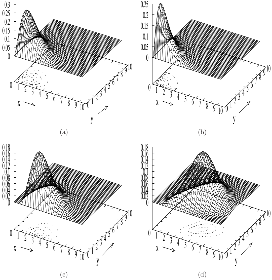
Figure 1: Surface plots of f_{X,Y}(x,y) for different values of \alpha_1, \alpha_2 and p , when \lambda_1 = \lambda_2 = 1 . (a) \alpha_1 = \alpha_2 = 2, p = 0.5 , (b) \alpha_1 = \alpha_2 = 2, p = 0.95 , (c) \alpha_1 = 10, \alpha_2 = 2, p = 0.5 , (d) \alpha_1 = 10, \alpha_2 = 2, p = 0.05 .
