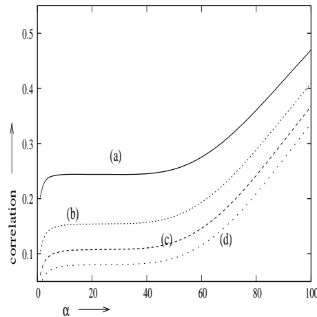
Figure 4: Correlation coefficient between X and Y for different values of \alpha and \lambda_3 when \lambda_1 = 1 , \lambda_2 = 1 : (a) \lambda_3 = 2.0 (b) \lambda_3 = 3.0 , (c) \lambda_3 = 4.0 , (d) \lambda_3 = 5.0 .
