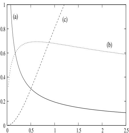
Figure 2: HF of WWE distribution for different values of \alpha and \beta when \lambda = 1 : (a) \alpha = 0.25 , \beta = 1.0 (b) \alpha = 0.75 , \beta = 5.0 , (c) \alpha = 1.5 , \beta = 0.1 .
