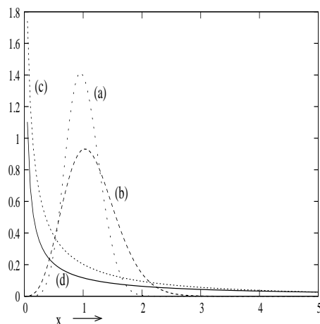
Figure 1: PDF of WWE distribution for different \alpha and \beta , when \lambda = 1 : (a) \alpha = 2 , \beta = 2 , (b) \alpha = 3 , \beta = 3 , (c) \alpha = 0.5 , \beta = 2 , (d) \alpha = 0.25 , \beta = 1 .
