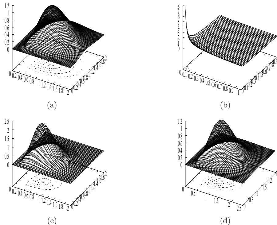
Figure 3: Surface plots of f_{X,Y}(x, y) for different values of \alpha , \lambda_1 , \lambda_2 and \lambda_3 . (a) \alpha_1 = 2.0 , \lambda_1 = \lambda_2 = 1 , \lambda_3 = 2.00 , (b) \alpha_1 = 0.25 , \lambda_1 = \lambda_2 = 1 , \lambda_3 = 2.00 , (c) \alpha_1 = \lambda_1 = \lambda_2 = \lambda_3 = 2.00 , (d) \alpha_1 = 2.0 , \lambda_1 = \lambda_2 = 1 , \lambda_3 = 0.25 .
