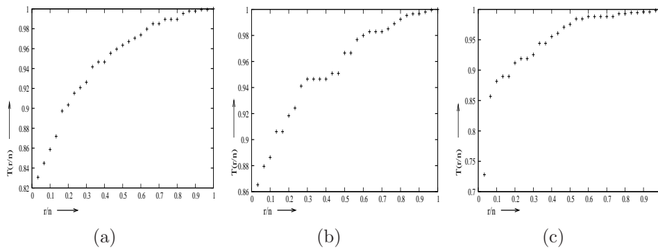
Figure 5: Scaled TTT transform of (a) X_1 (b) X_2 (c) X_3 .
