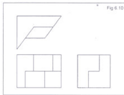
Home Assignment No. 6, Solution - Missing Views and Lines
