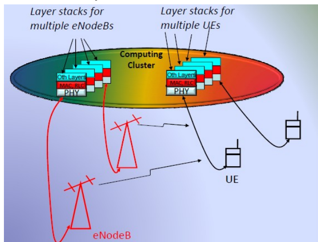
Fig.3. Flow-diagram for the centralized processing
