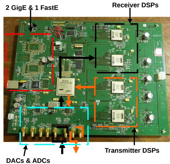
Fig.6. Picture of the prototype Baseband section
