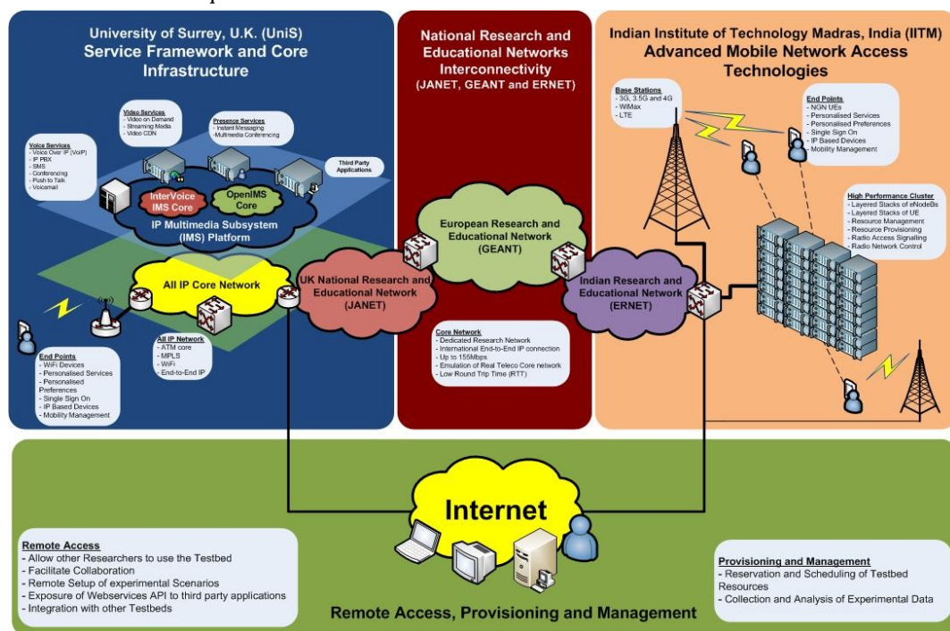
Fig.7. High level integrated view of Access, Core and Service delivery testbed
