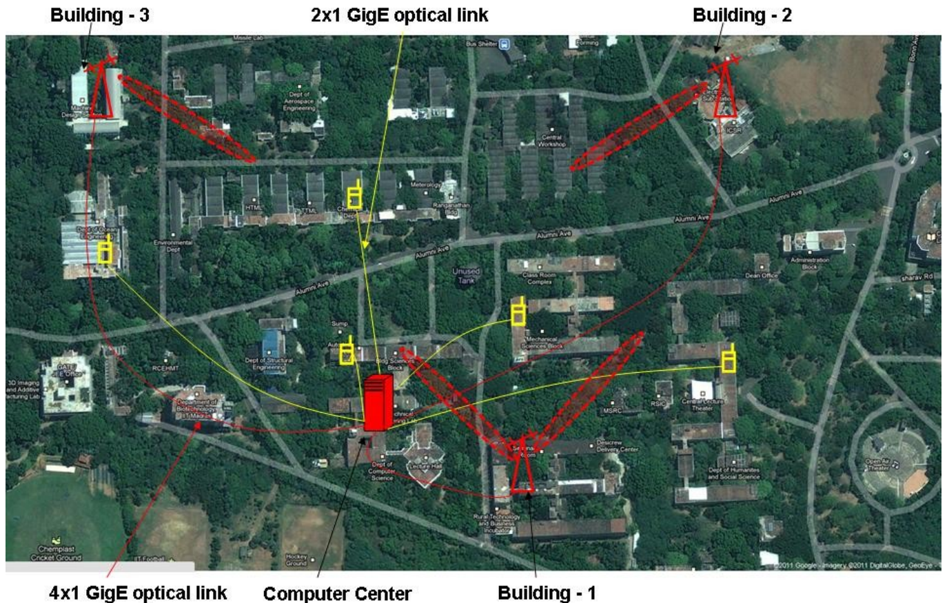
Fig.1. Layout of the IITM Access-network testbed
