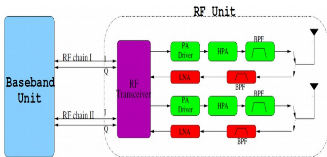
Fig.2. Block-diagram of the Baseband and RF unit
