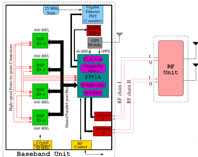
Fig.5. Block diagram of Baseband unit
