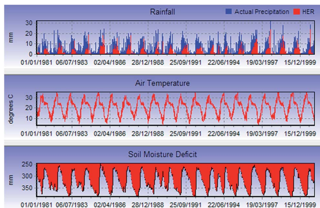
Fig. 8 Daily precipitation, HER, temperature and SMD for the Ganga basin over the period 1981–2000.
