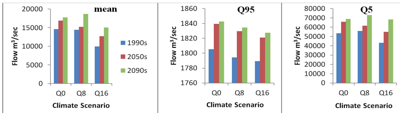
Fig. 16 Annual mean, Q95 and Q5 flows for baseline 1990s, 2050s and 2090s under the three climate change realizations Q0, Q8 and Q16.
