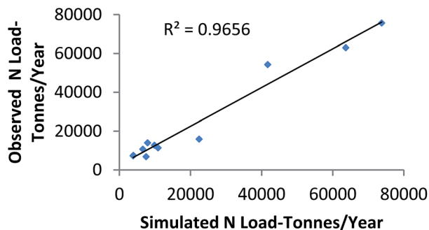
Fig. 12 Simulated and observed nitrogen load in the Ganga river at Kanpur.
