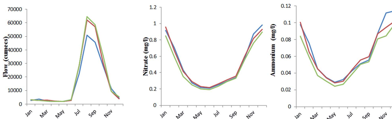
Fig. 13 Effects of climate change on monthly mean Farakka Ganga flow, and nitrate and ammonia concentrations for baseline 1990s (blue), 2050s (red) and 2090s (green) under climate scenario Q0.
