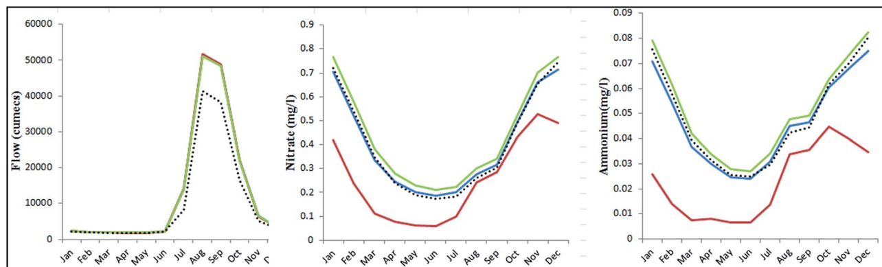
Fig. 17 Mean monthly flow, and nitrate and ammonia concentrations 2050s means for the three SSPs (blue-BaU, red-MS, green-LS) compared to the baseline 1990s (dotted line), assuming the Q16 climate change scenario.
