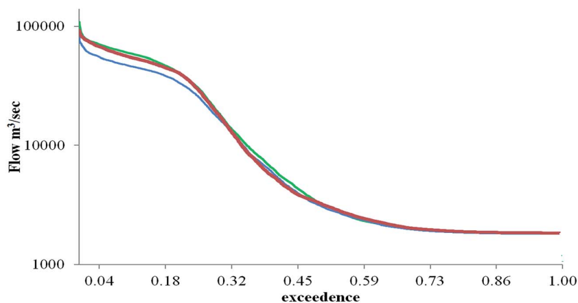
Fig. 14 Flow duration curves for 1990s (blue), 2050s (green) and 2090s (red) for the lower Ganga river at Farakka under the climate realization Q0.
