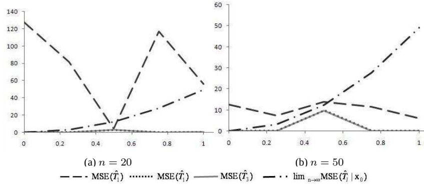
Figure 8: MSE of \hat{T}_1, \hat{T}_2, \hat{T}_3 in case of normal distribution with \sigma_\epsilon^2 = 0.5, \sigma_\phi^2 = 0.5, \sigma_\delta^2 = 1.25
