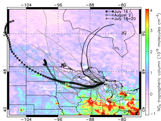
Fig. 5. The SCIAMACHY-retrieved 0.25 degree gridded tropospheric \text{NO}_2 column data from June–August 2009. The locations of the UMBS site and the nearby large urban centers are shown by white open diamonds. The white open square shows the location of the SPP, which was ranked 29th in US Environmental Protection Agency (EPA) region 5 (IL, IN, MI, MN, OH and WI) in 2009 for \text{SO}_2 emissions (24015.8 tons) and 6th by \text{NO}_x (13873.7 tons) under Acid Rain Program (ARP) sources ( http://camddataandmaps.epa.gov/gdm/ ). The HYSPLIT-calculated 3-day backward trajectories starting at 10 m at 19:00 LT from 8 July–2 August are also shown, highlighting the two early evening NPF events on 16 July (black line with stars) and 2 August (black line with open diamonds) and very clean non-event days (18–20 July) (black line with plus sign).
