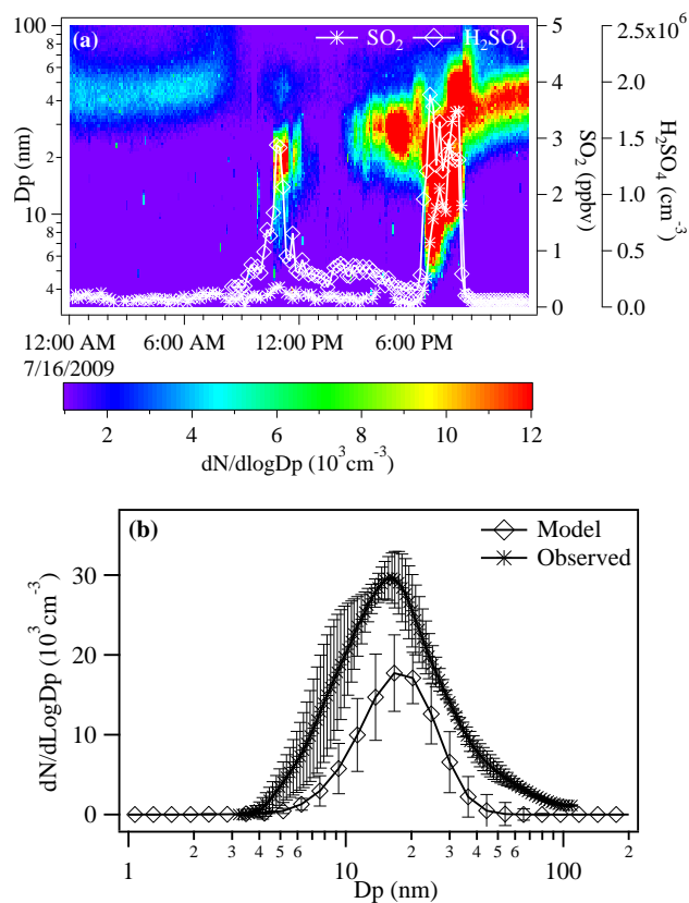
Fig. 4. (a) Particle number size distributions, \text{SO}_2 (white asterisks) and \text{H}_2\text{SO}_4 (white open diamonds) measured on 16 July 2009. The 2 August evening event also showed a strikingly similar feature as here. (b) The size distributions predicted from the model at the end of 35 h simulation (line with open diamonds) and that measured at the forest site at 19:00 LT (line with asterisks). The vertical bars indicate one standard deviation values. Considering uncertainties in measurements and modeling simulations, this is a very good agreement. IIN simulations for the 2 August event also showed very similar results.
