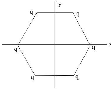
Figure 2: Charges at the corners of a hexagon.
