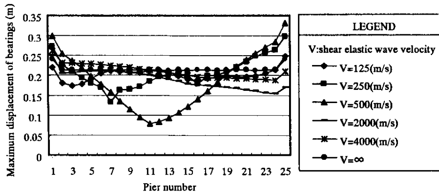
Fig. 14 Maximum displacement of bearings caused by difference of phase of inputs
