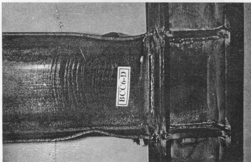
Fig. 15(a) Fracture in the beam flange along the weld line (BCC6)
