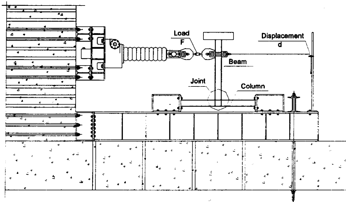
Fig. 4 Experimental set-up
