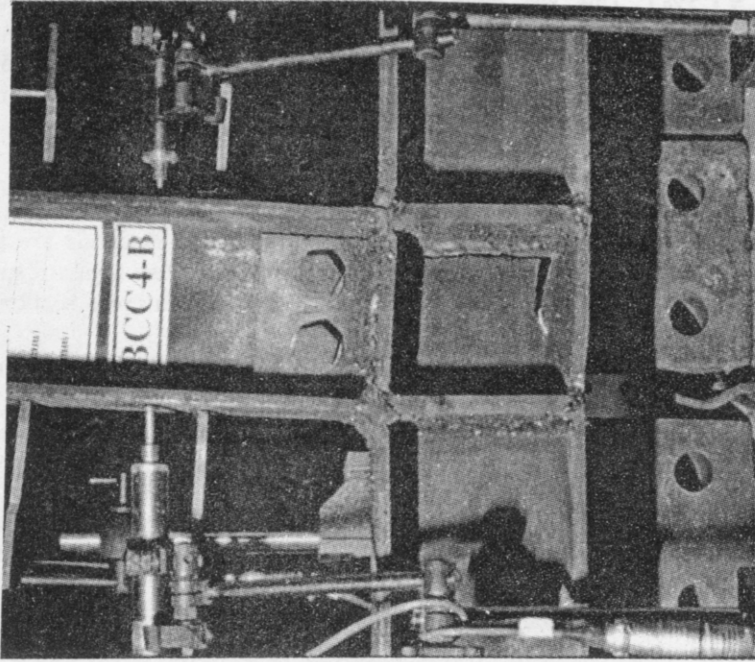
Fig. 11 Failure mode of the panel zone of a welded flange and web cleats connection (BCC4)
