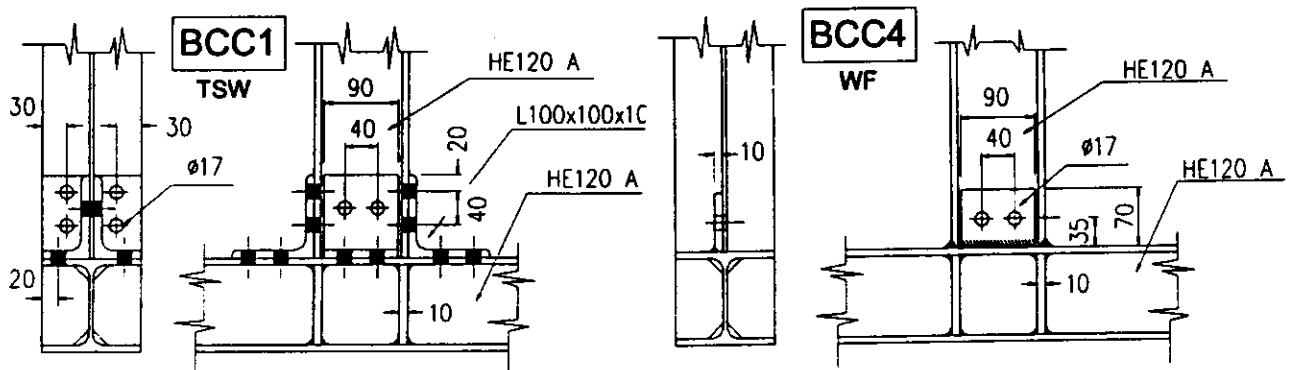
Fig. 1 Small-scale specimens
