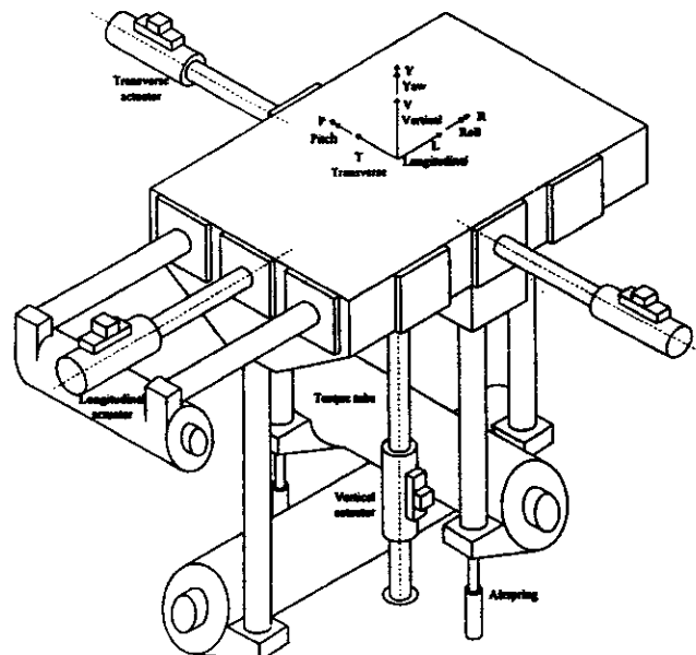
Fig. 1 General perspective of LNEC shaking table (Crewe, 1997)
