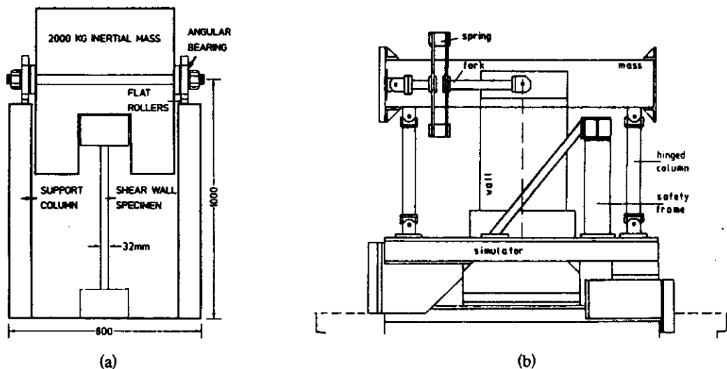
Fig. 3 Testing of RC walls using auxiliary frames to support inertia masses: (a) Elnashai et al. (1988) (b) Rothe and König (1988)
