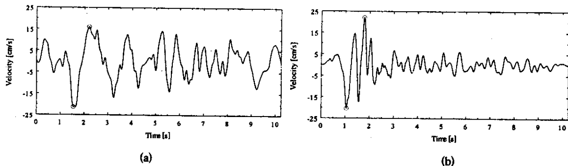
Fig. 21 Velocity time-history for (a) artificial record (b) natural record
