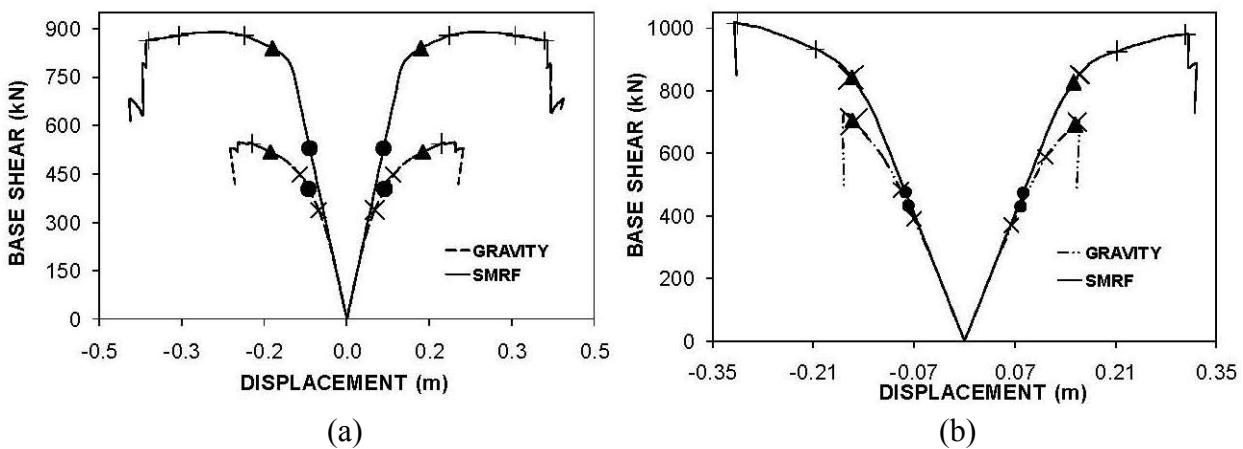
Fig. 3 Comparison of capacity curves and performance points for the 4-storey building designed for gravity and as SMRF, as per the relevant Indian standard (the dot (●) represents the performance point for DBE, and triangle (▲) represents the performance point for MCE; the three crosses (+) represent the IO, LS, and CP performance levels, consecutively): (a) longitudinal direction; (b) transverse direction
