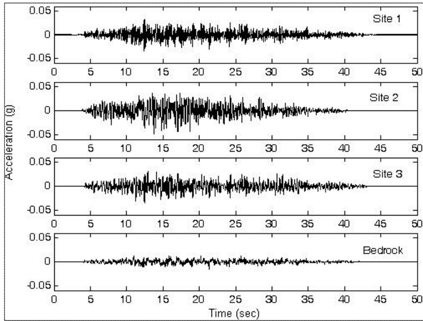
Fig. 4 Bedrock level and free-field motions at the top of three sites for a simulation of earthquake with M_w = 7.5
