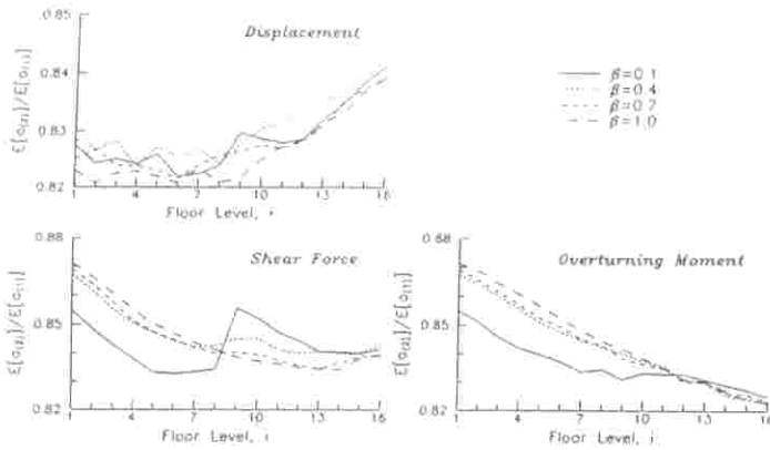
Fig. 6 Effects of floor mass and story stiffness distribution in case of step reduction by factor \beta .
