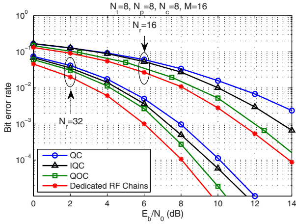
Fig. 2. Combining schemes for N_r = 16 and 32.
