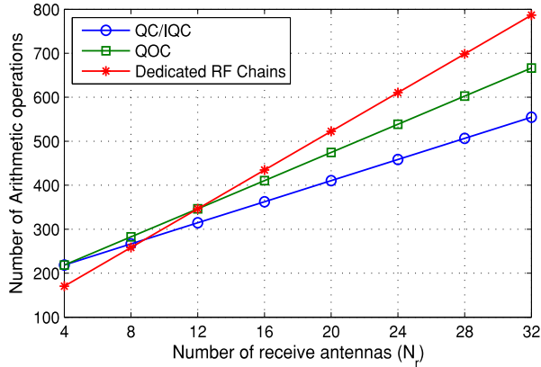
Fig. 7. Number of arithmetic operations per bit required with MMSE detection for N_c = N_t = 4 , N_p = 4 and M = 4 at E_b/N_0 = 6 dB.
