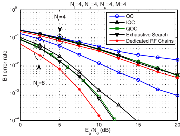
Fig. 3. Combining schemes for N_r = 4 and 8.
