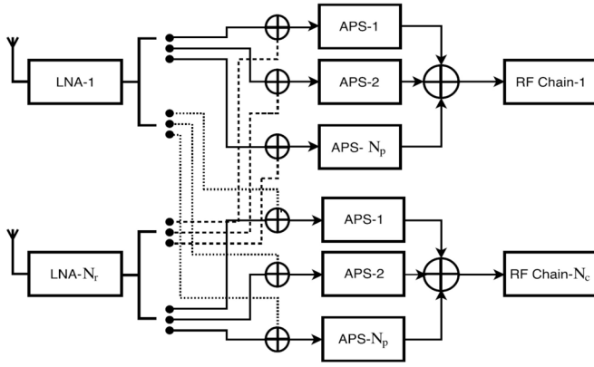
Fig. 1. Massive MIMO combining architecture for reducing RF chains [9].
