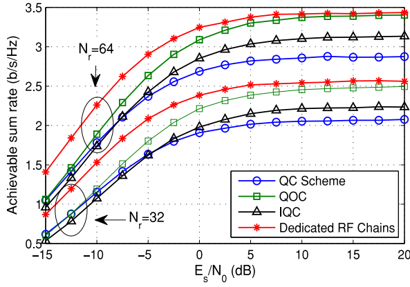
Fig. 6. Sum rate per transmit antenna for N_c = N_t = 8 and N_p = 4 .
