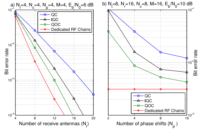
Fig. 5. BER performance of the combining schemes using MMSE detection with increasing number of receive antennas/APs.
