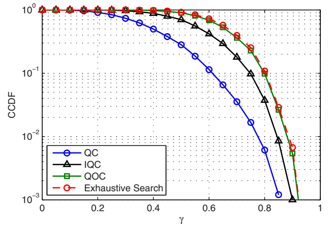
Fig. 4. CCDF of \text{Orth}(\mathbf{C}) .
