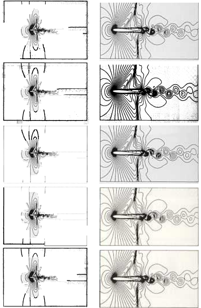
Fig. 9. Mach = 0.85, Re = 10,000, \alpha = 2^\circ , H = 4.25 flow past a NACA0012 airfoil: density field at five instants during one cycle of lift coefficient for the temporally periodic solution
