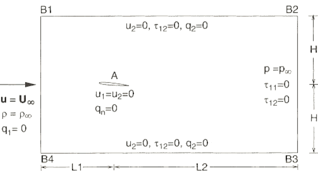
Fig. 3. Flow past an airfoil in a channel problem description
