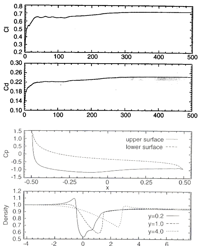
Fig. 17. Mach = 0.85, Re = 10,000, \alpha = 8^\circ , H = 4.25 flow past a NACA0012 airfoil: time histories of the lift and drag coefficients, C_p distribution on the airfoil surface and the stream-wise variation of density in the domain at three vertical locations for the steady-state solution
