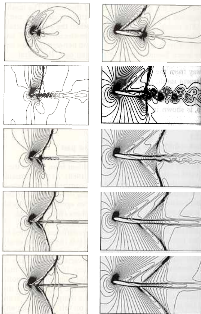
Fig. 18. Mach = 0.85, Re = 10,000, \alpha = 10^\circ , H = 4.25 flow past a NACA0012 airfoil: density field at t = 3.6, 50.3, 100.3, 120.3, 150.3
