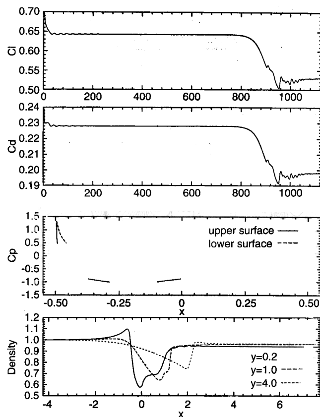
Fig. 24. Mach = 0.85 , Re = 10,000 , \alpha = 7^\circ , H = 4.25 flow past a NACA0012 airfoil: time histories of the lift and drag coefficients, C_p distribution on the airfoil surface and the stream-wise variation of density in the domain at three vertical locations for the solution at t = 1100 . The steady-state solution at \alpha = 8^\circ (see Fig. 21) is used as an initial condition
