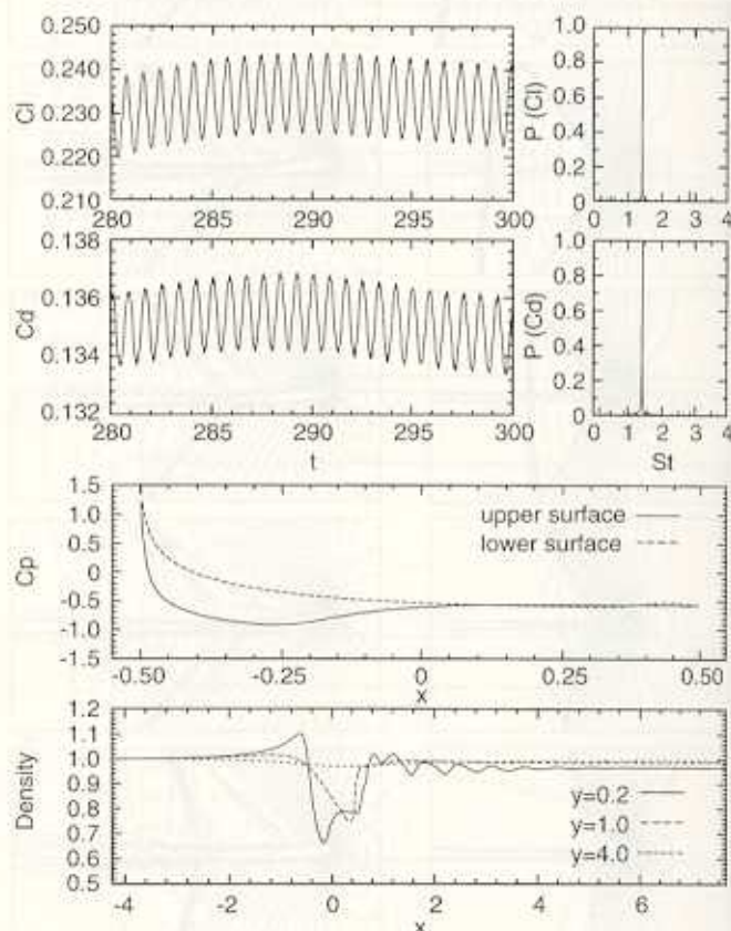
Fig. 26. Mach = 0.85 , Re = 10,000 , \alpha = 5^\circ , H = 12 flow past a NACA0012 airfoil: time histories of the lift and drag coefficients, their power spectra, the C_p distribution on the airfoil surface and the stream-wise variation of the density at various vertical locations corresponding to the peak value of the lift coefficient
