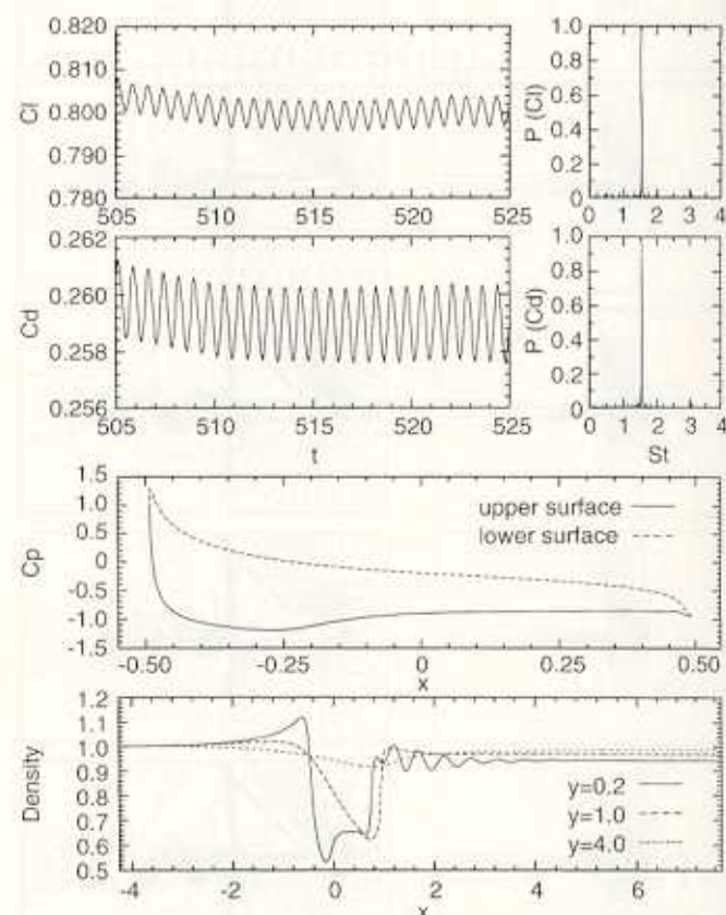
Fig. 30. Mach = 0.85, Re = 10,000, \alpha = 10^\circ , H = 12 flow past a NACA0012 airfoil: time histories of the lift and drag coefficients, their power spectra, the C_p distribution on the airfoil surface and the stream-wise variation of the density at various vertical locations corresponding to the peak value of the lift coefficient
