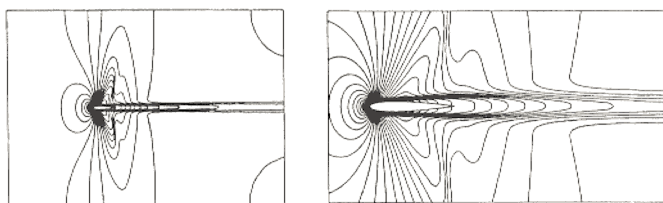
Fig. 5. Mach = 0.85, Re = 2000, \alpha = 0^\circ flow past a NACA0012 airfoil: density field for the steady-state solution
