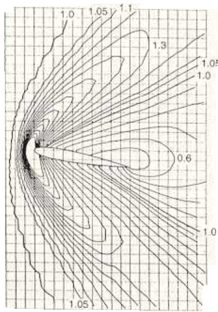
Fig. 2. M = 2.0 , Re = 106 , \alpha = 10^\circ flow past a NACA0012 airfoil: density field for the steady-state solution; measurements (left) from Allegre et al. and numerical results (right) from Haase (1987)
