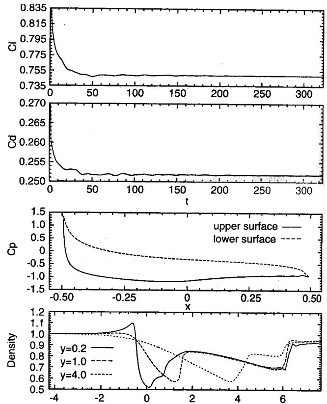
Fig. 22. Mach = 0.85, Re = 10,000, \alpha = 8^\circ , H = 4.25 flow past a NACA0012 airfoil: time histories of the lift and drag coefficients, C_p distribution on the airfoil surface and the stream-wise variation of density in the domain at three vertical locations for the steady-state solution. The steady-state solution at \alpha = 10^\circ (see Fig. 19) is used as an initial condition
