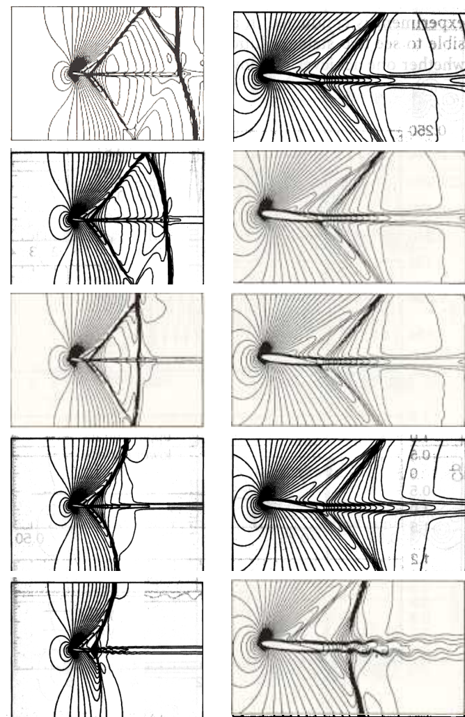
Fig. 23. Mach = 0.85 , Re = 10,000 , \alpha = 7^\circ , H = 4.25 flow past a NACA0012 airfoil: density field at t = 20.0, 296.4, 590.2, 798.5, 1118.5 . The steady-state solution at \alpha = 8^\circ (see Fig. 21) is used as an initial condition
