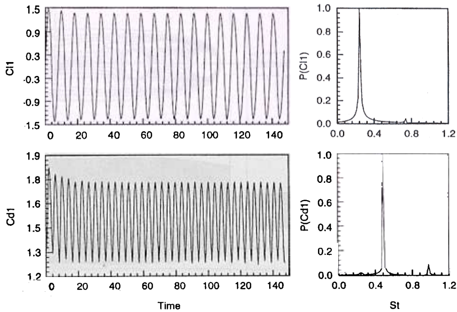
Figure 5. Re 1000 flow past a single cylinder: time histories of lift and drag coefficients and their power spectra
