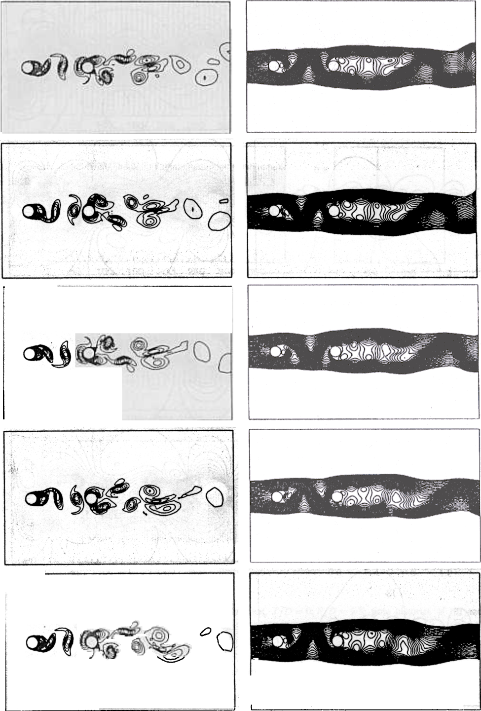
Figure 15. Re\ 1000 flow past two cylinders in tandem arrangement, T/D = 0 , P/D = 5.5 : vorticity and streamfunction fields at five instants during one period of lift coefficient for upstream cylinder
