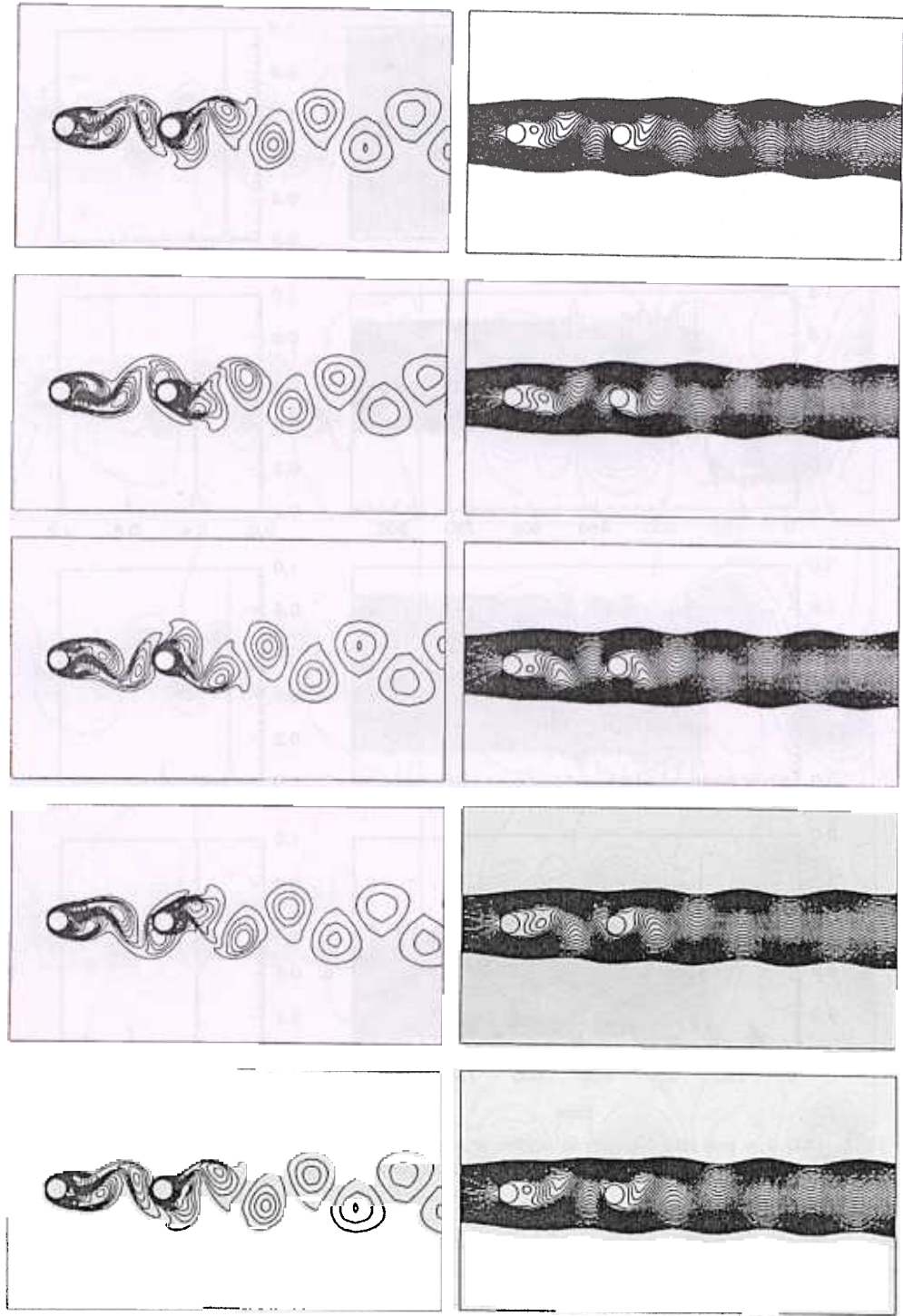
Figure 12. Re\ 100 flow past two cylinders in tandem arrangement, T/D = 0 , P/D = 5.5 : vorticity and streamfunction fields at five instants during one period of lift coefficient for upstream cylinder
