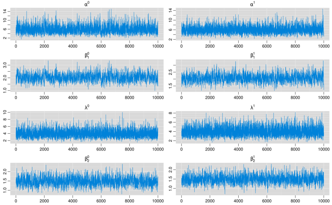
Figure 9. Trace plots of the posterior distributions of the parameters.
