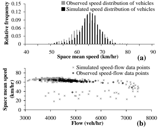
Figure 2: Comparison of (a) speed distribution and (b) speed-flow relation obtained from traffic stream at Delhi-Gurgaon highway, NH-8, (without lane discipline and with 70% passenger-car and 30% motorized two wheelers) with those obtained from a CUTSiM simulation of a similar stream.
