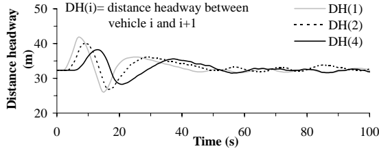
Figure 1: Study of asymptotic stability of a single lane traffic stream simulated using CUTSiM.
