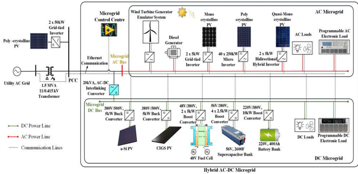
Fig.1: Schematic block diagram of the system architecture
