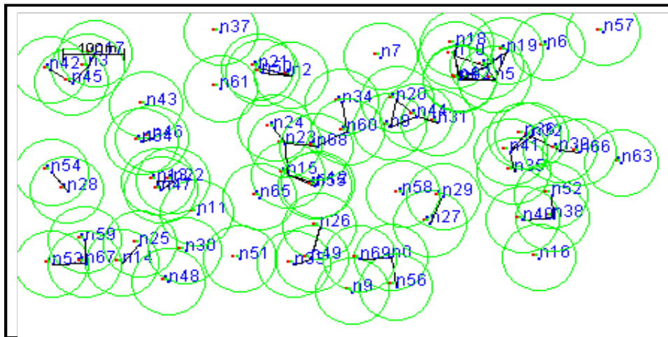
Figure 3.2: Cluster formation
